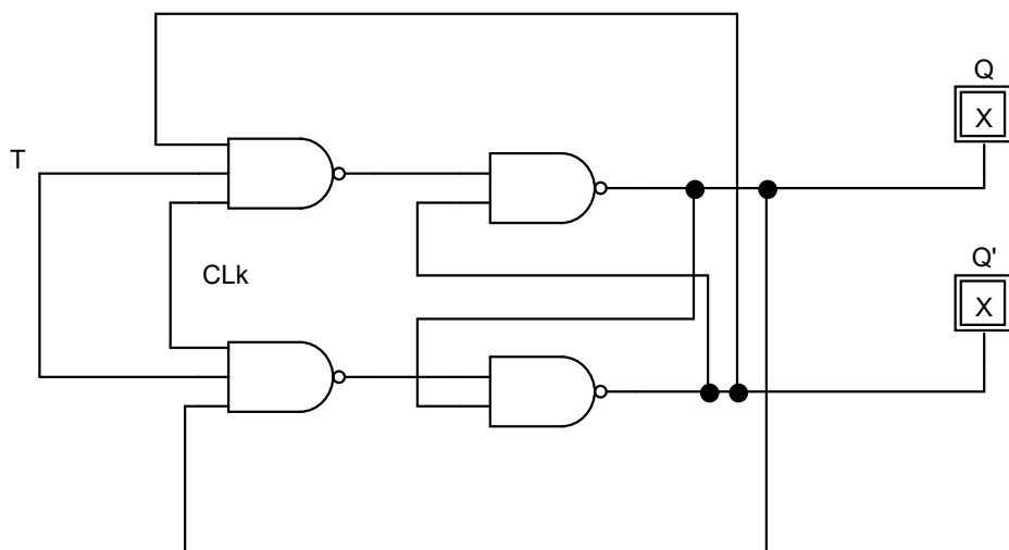
T flip flop
