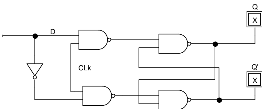
D flip flop
